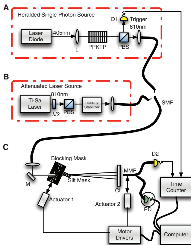
Fig. 2. Experimental setup used for the measurement of \kappa . (A) Creation of heralded single photons from a periodically poled potassium titanyl phosphate (PPKTP) nonlinear crystal pumped by a 405-nm laser diode. Parametric downconverted photons are emitted as pairs at 810 nm and are coupled into a single-mode fiber (SMF). Photon detection (D1) in the trigger output heralds a single photon, which is then sent through the diffraction slits. (B) A pulsed titanium-sapphire (Ti-Sa) laser is attenuated and coupled into a SMF. The attenuation is realized by the combination of a half-wave plate ( \lambda/2 ) and a polarizing beamsplitter (PBS), combined with neutral filters and an intensity stabilizer. (C) Schematic of the three-slit experiment where the photons from the source go through the movable blocking mask with the eight combinations and then through
