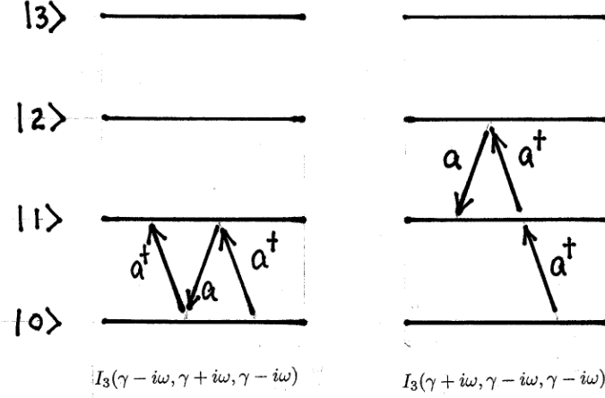
Figure 1: Application of diagrammatic rules to two third-order terms in the perturbation series expansion of the harmonic oscillator driven by a decaying exponential dipole interaction.
